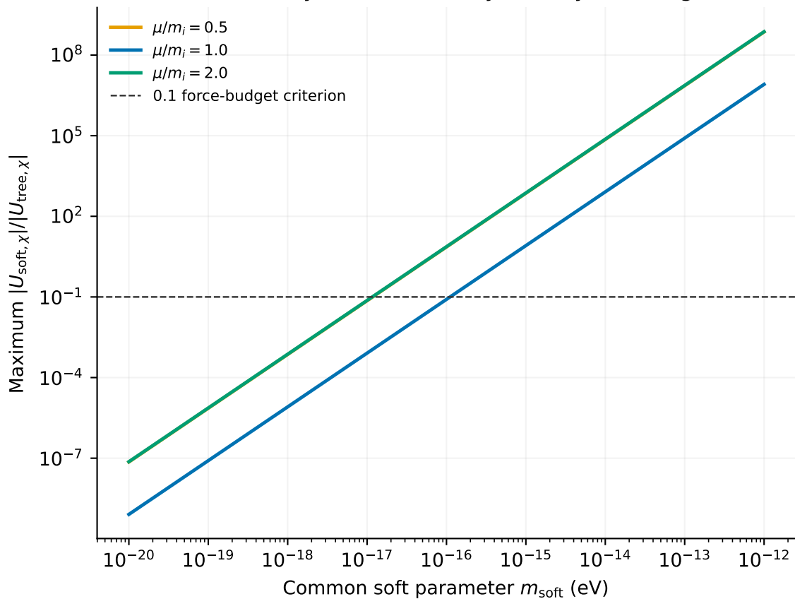
Sensitivity to additional symmetry breaking
