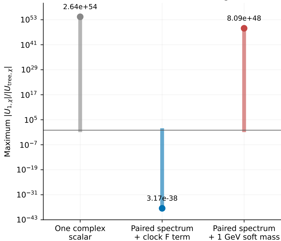
100 GeV: conditional force budgets
