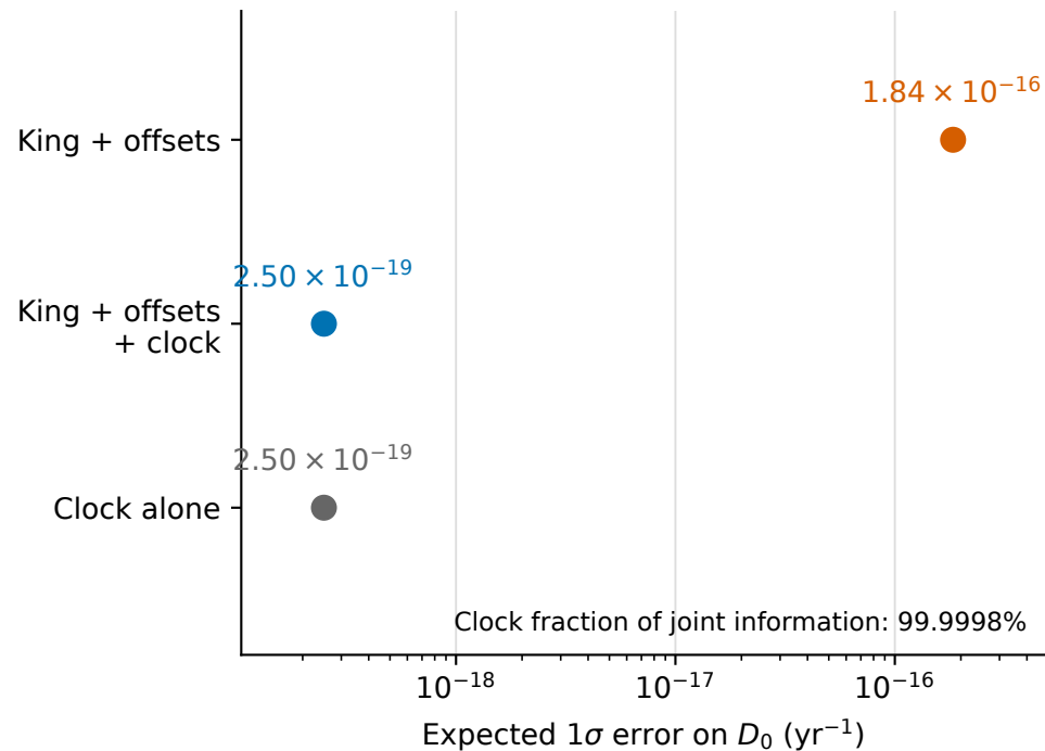
(b) Drift precision, fixed s = 2
