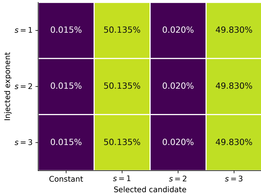
(a) AIC selection frequencies d = +12.5 : five clock standard errors
