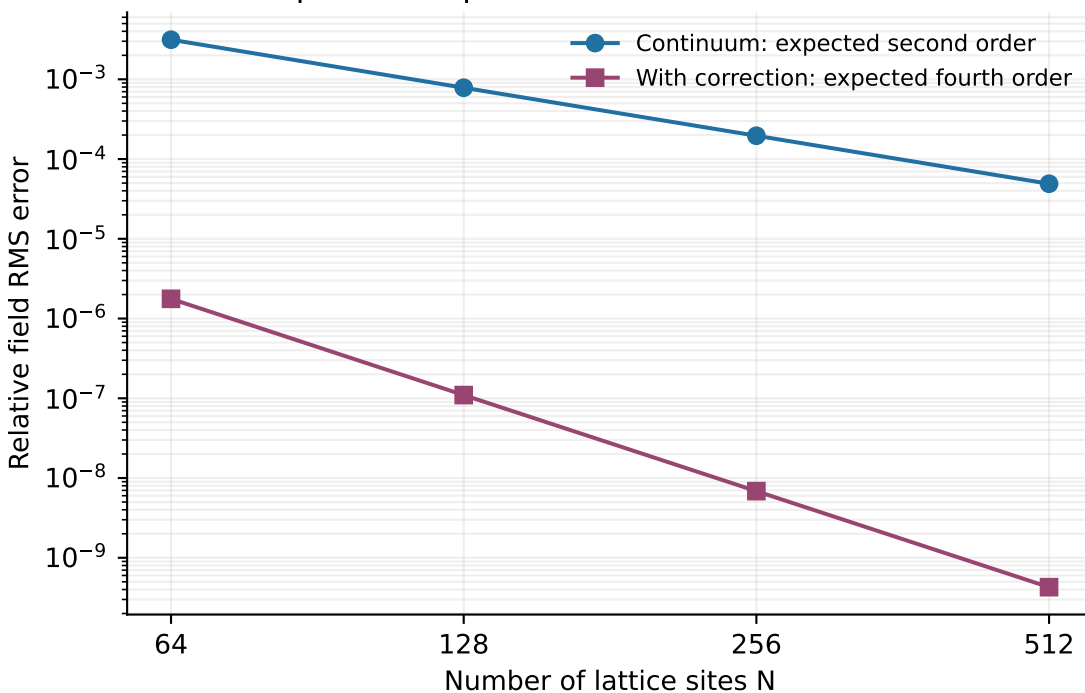
Long-wave expansion fails near grid scales
