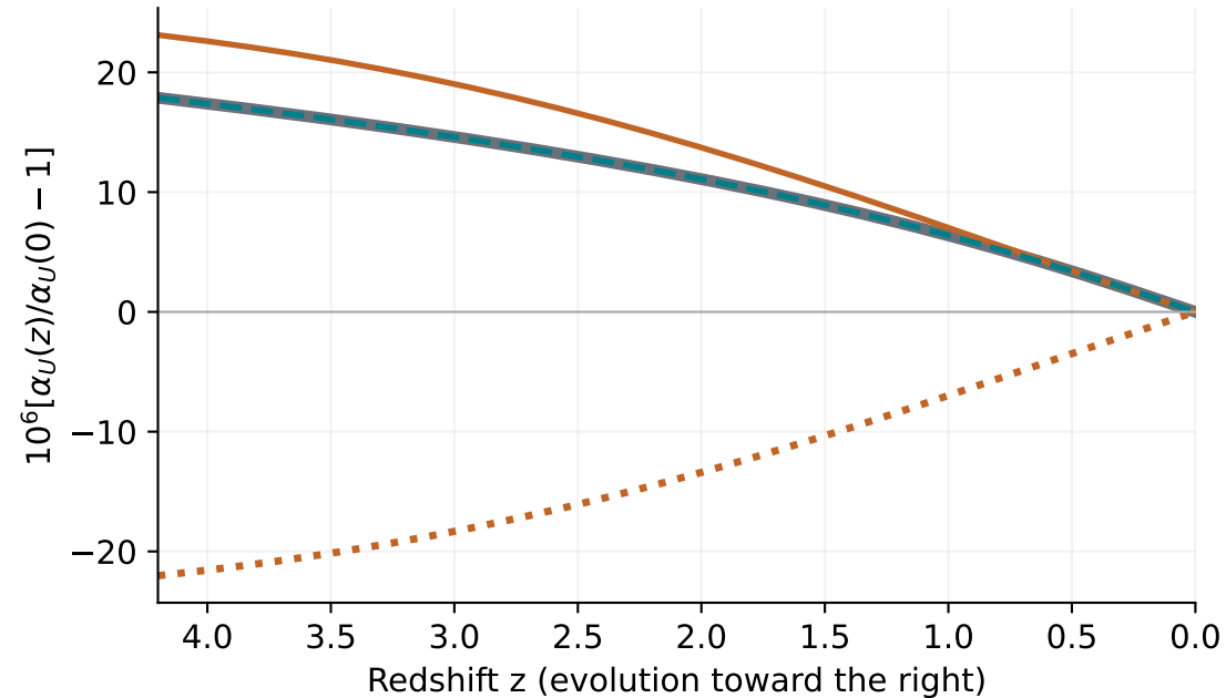
(a) UV boundary determines the comparison
