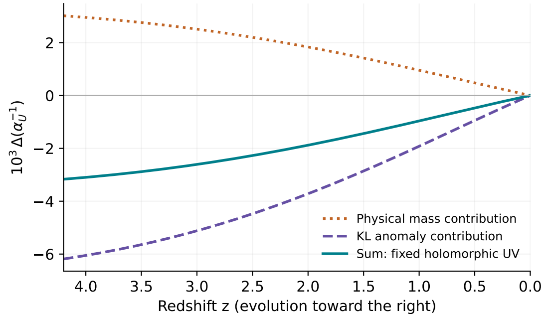
(b) Canonical K: terms in the inverse coupling
