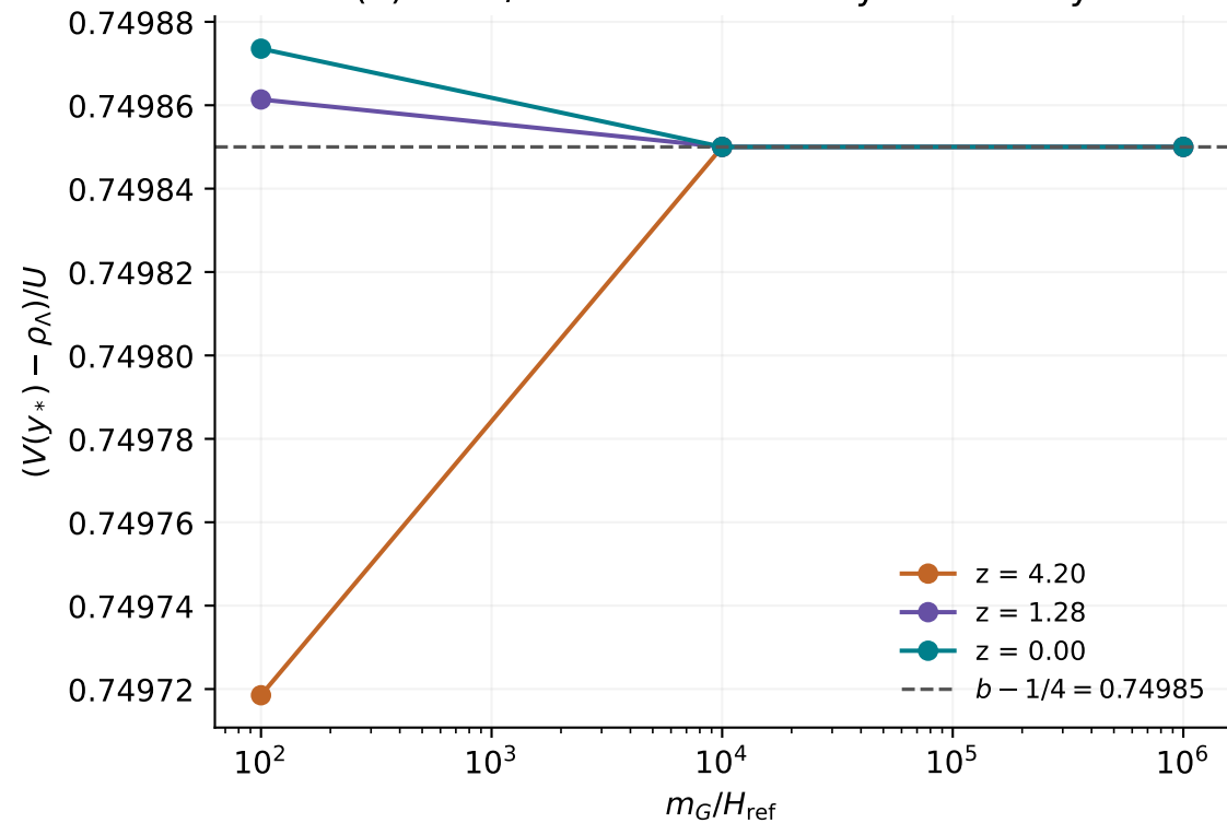
(a) \theta = \pi/2 : a classical heavy-field valley
