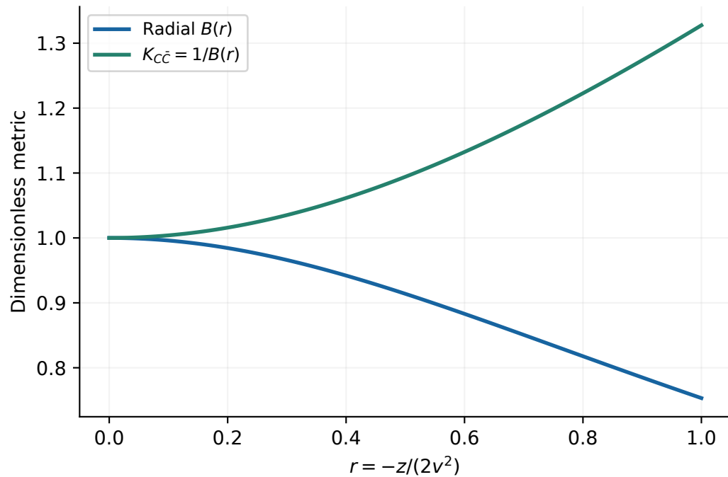
(c) Zero-source quotient geometry
