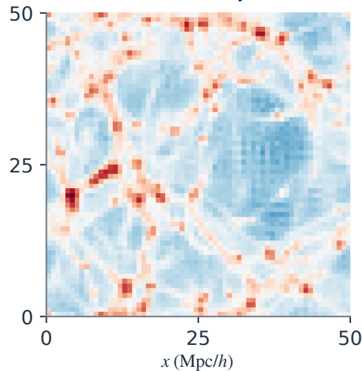
(f) a=1 , z=0 t=13.790 Gyr
