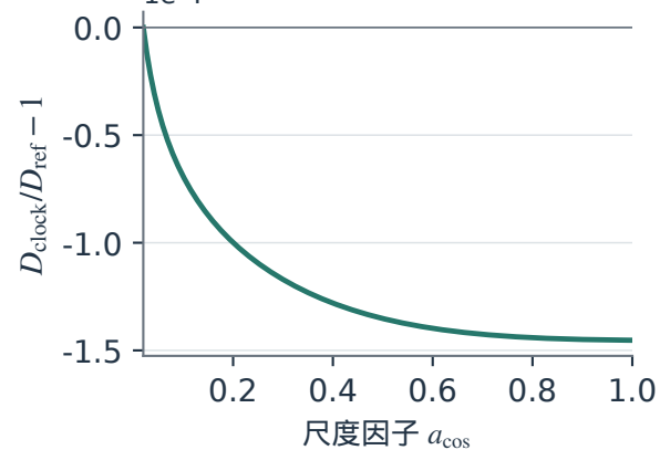
(f) a=1 , z=0 t=13.790 Gyr
