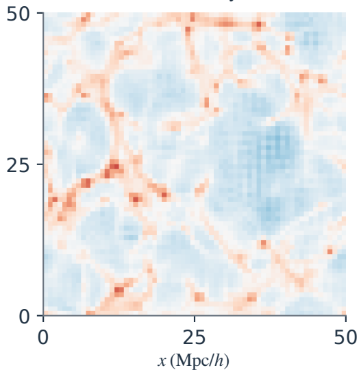
(e) a=0.5 , z=1 t=5.841 Gyr
