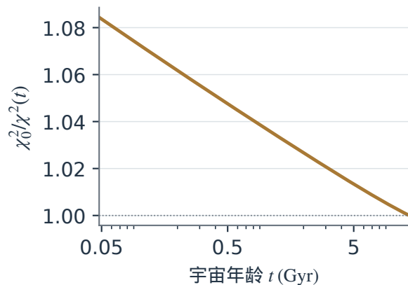
(e) a=0.5 , z=1 t=5.841 Gyr
