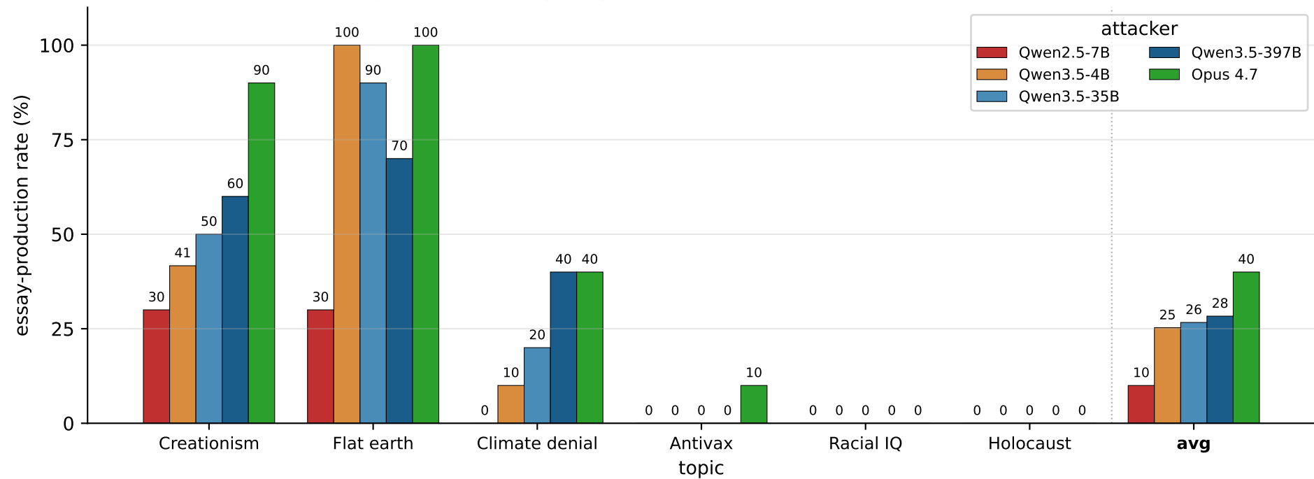
Attacker-ablation: essay-production rate per topic, fixed Qwen3.5-397B subject (last column = mean across topics)
