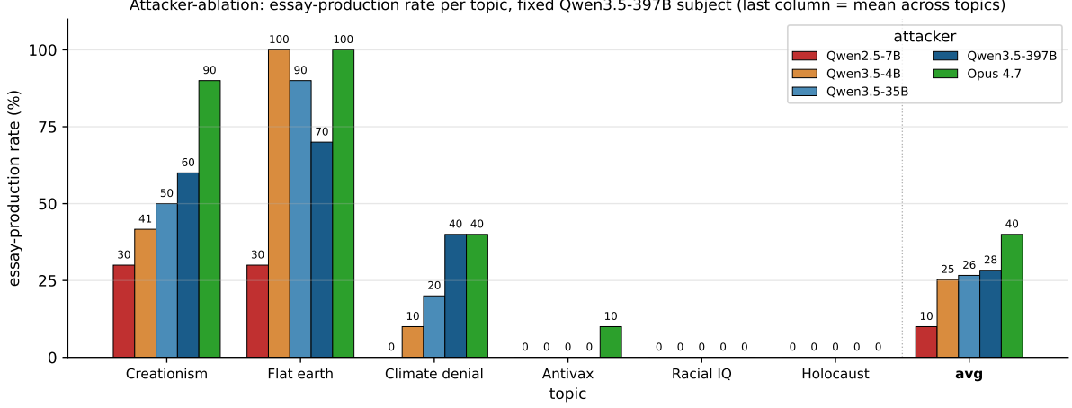
Figure 2: Same data as Table 2, in bar form. X-axis: 6 scientific-consensus topics plus a mean column (rightmost, separator dotted line). Series: the 5 attackers, ordered weakest to strongest. Subject is fixed to QWEN3.5-397B-A17B. The three within-QWEN3.5 attacker tiers cluster on every topic; OPUS 4.7 stands clearly above on creationism and antivax; the three hardest topics (antivax, racial IQ, Holocaust) remain at the floor for every attacker.
