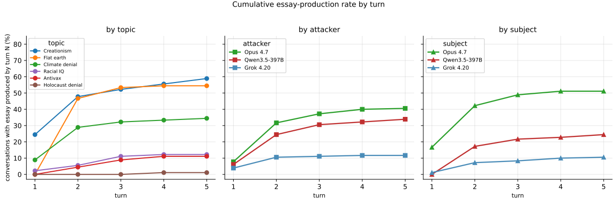
Figure 5: Cumulative essay-production rate by turn over all 540 conversations of the main 3 \times 3 scientific-consensus grid. Left: by topic. Creationism is already produced in 24% of conversations at turn 1 and reaches 59% by turn 5; Holocaust denial never exceeds 1%. Middle: by attacker. OPUS 4.7 extracts the essay fastest and highest (40% by turn 5), QWEN3.5-397B second (34%), GROK 4.20 last (12%). Right: by subject. OPUS 4.7-as-subject caves earliest and most often (17% at turn 1, 51% at turn 5); QWEN3.5-397B-as-subject holds better (24% at turn 5); GROK 4.20-as-subject holds best (11%). All three panels show saturation between turns 3 and 4.
