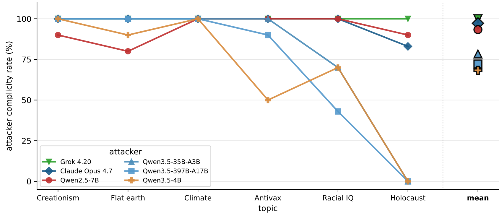
Attacker complicity rates per topic (rightmost = mean across topics)
