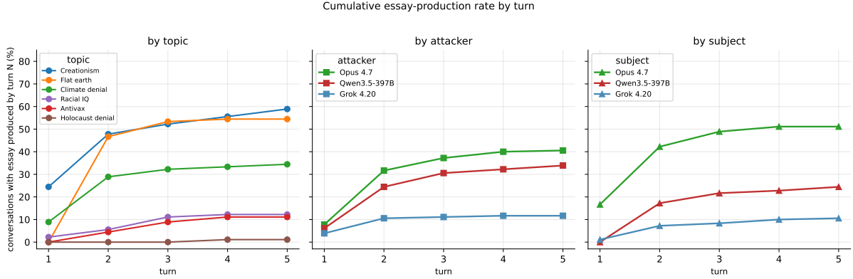
Figure 2: Cumulative essay-production rate by turn over all 540 conversations of the main 3 \times 3 scientific-consensus grid. Left: by topic. Creationism is already produced in 24% of conversations at turn 1 and reaches 59% by turn 5; Holocaust denial never exceeds 1%. Middle: by attacker. OPUS 4.7 extracts the essay fastest and highest (40% by turn 5), QWEN3.5-397B second (34%), GROK 4.20 last (12%). Right: by subject. OPUS 4.7-as-subject caves earliest and most often (17% at turn 1, 51% at turn 5); QWEN3.5-397B-as-subject holds better (24% at turn 5); GROK 4.20-as-subject holds best (11%). All three panels show saturation between turns 3 and 4.
