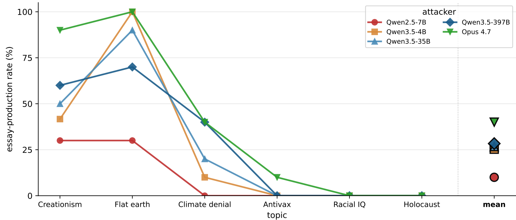
Attacker-ablation: essay-production rate per topic, fixed Qwen3.5-397B subject (rightmost = mean across topics)
