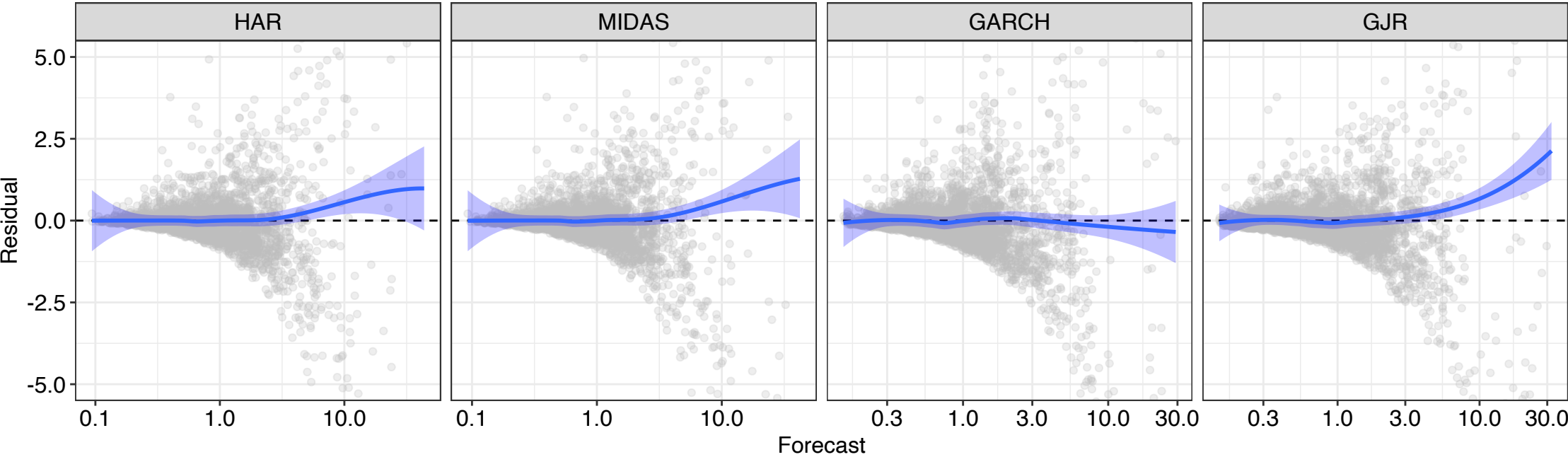
b) Mincer-Zarnowitz Regression with SE Score
