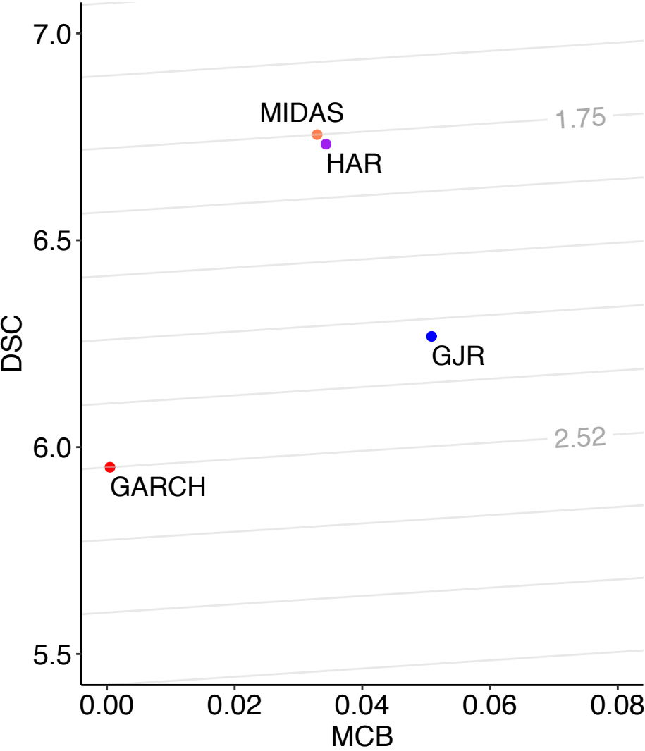
a) QLIKE Score
