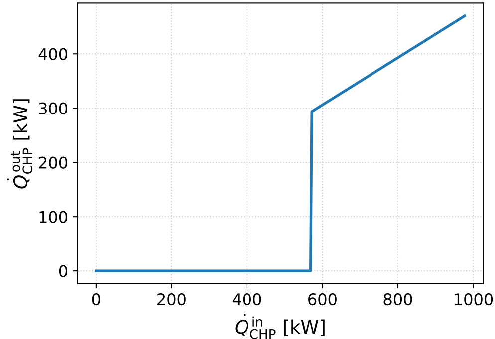
CHP heat
