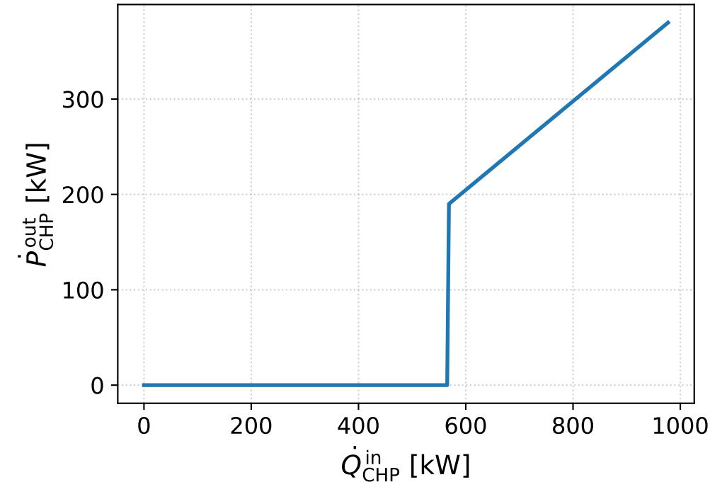
CHP electricity
