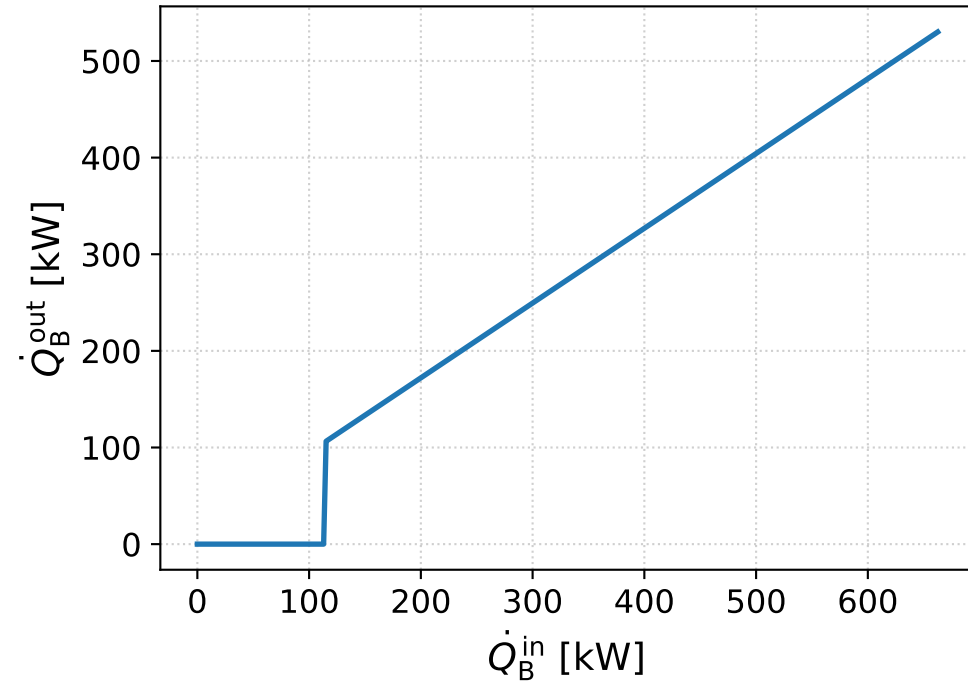
Boiler heat
