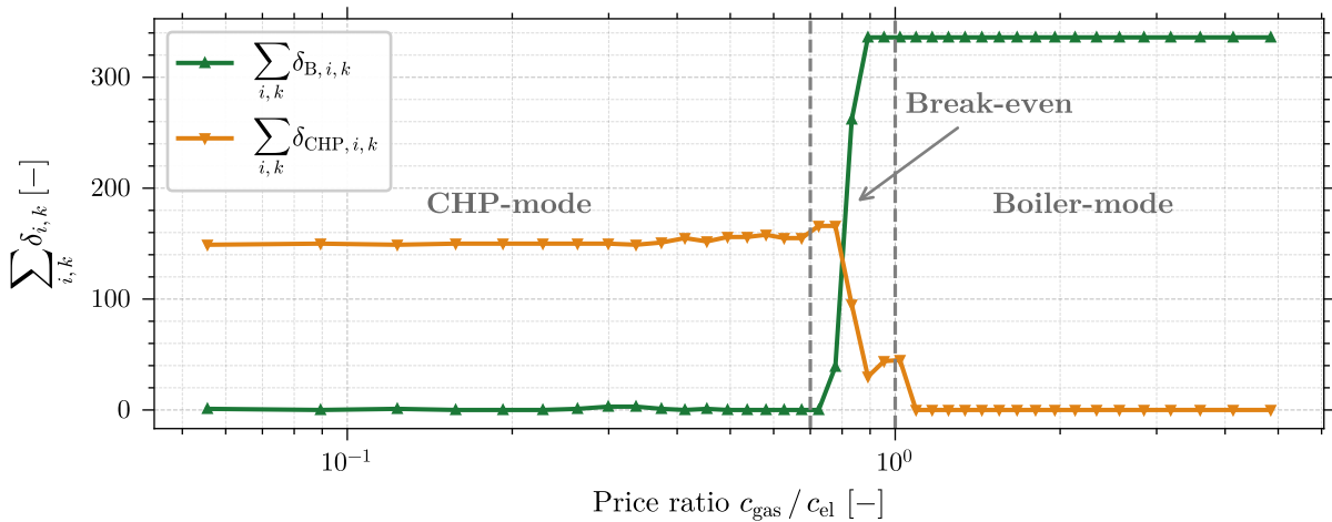
MILP Commitment: \sum_{i,k} \delta_{B,i,k} and \sum_{i,k} \delta_{CHP,i,k} vs Price Ratio
