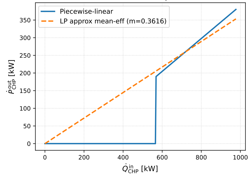
CHP electricity
