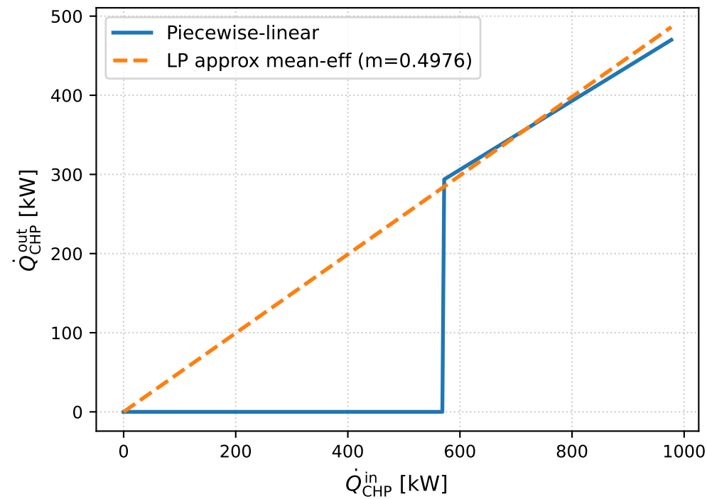
CHP heat
