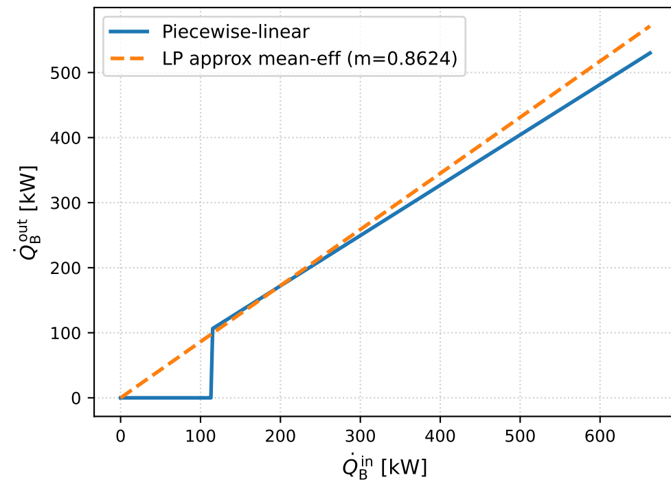
Boiler heat
