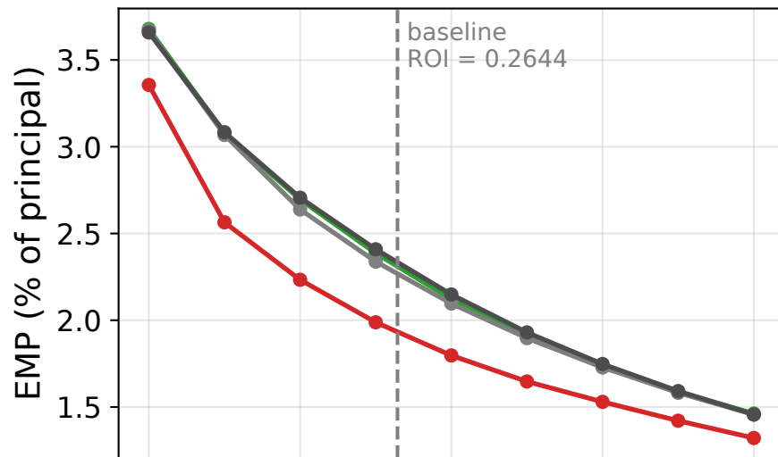
Taiwan (n = 30k)
