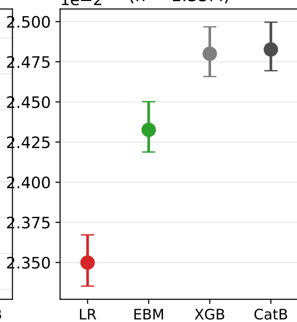
Lending Club (n = 1.35M)
