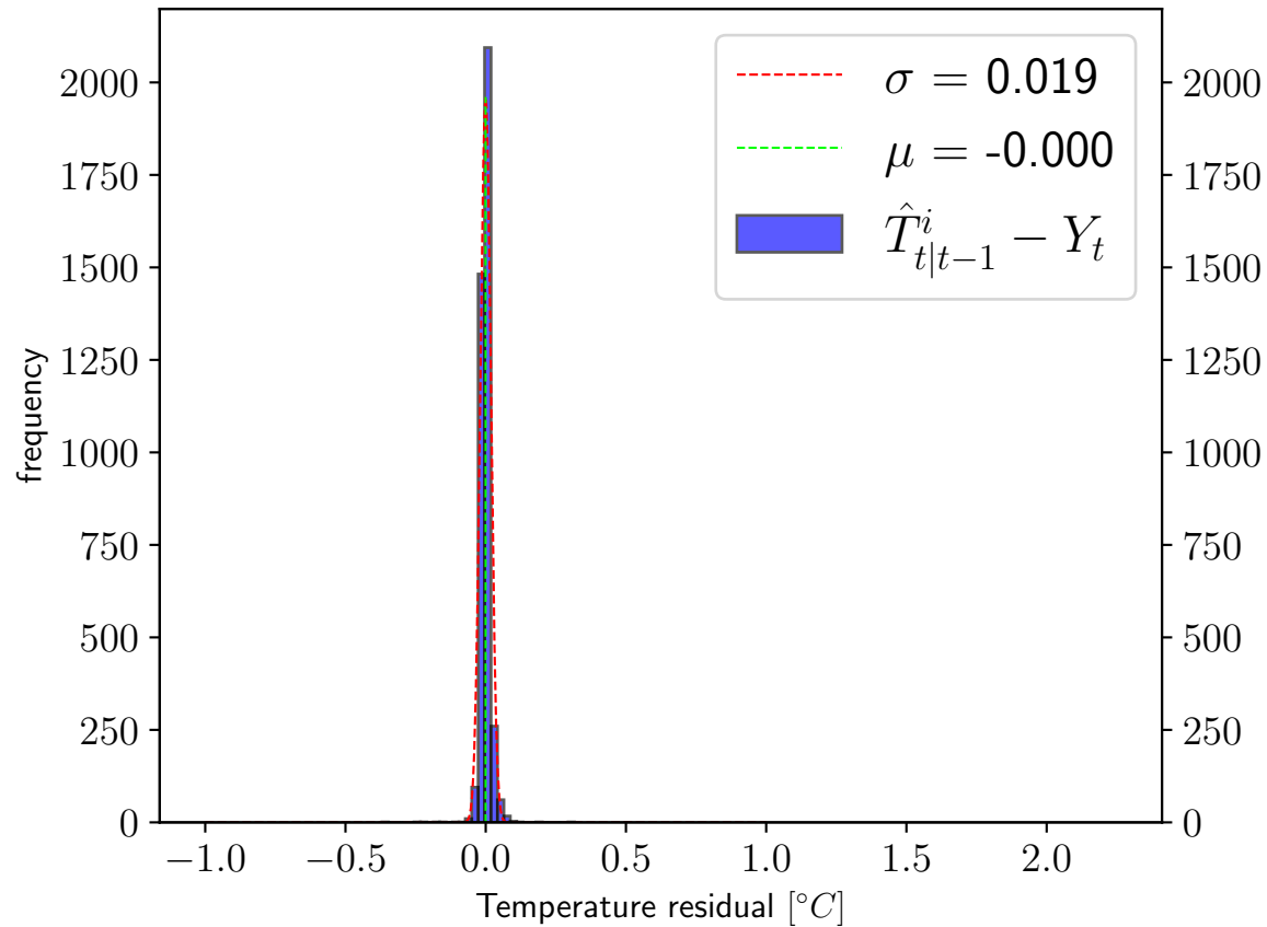
One-step ahead
