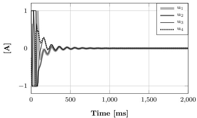
Solenoid Currents
