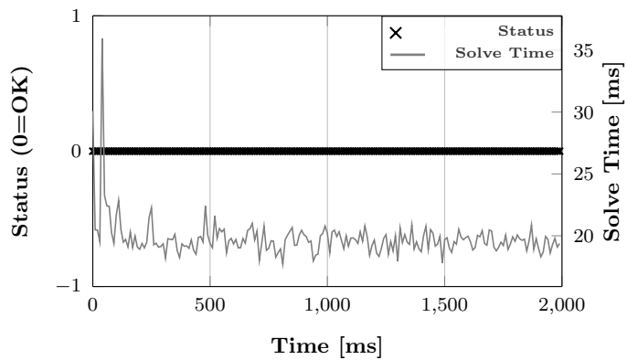
Solver Performance
