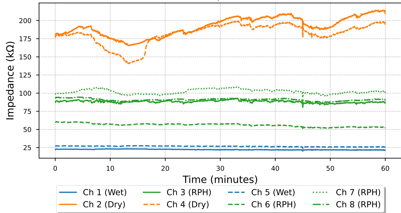
Individual Electrode Impedance Over One Hour
