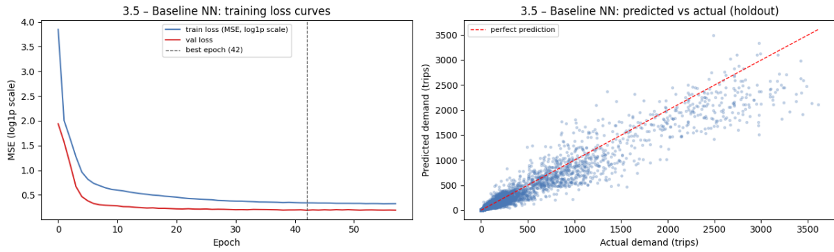
Figure 11: Training result of the baseline neural network, before hyperparameter tuning.
