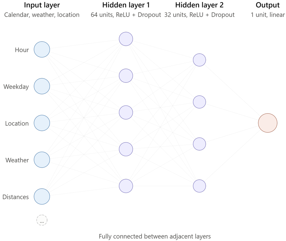
Figure 10: Architecture of the baseline neural network, showing layer sizes and the arrangement of the feedforward stack.
