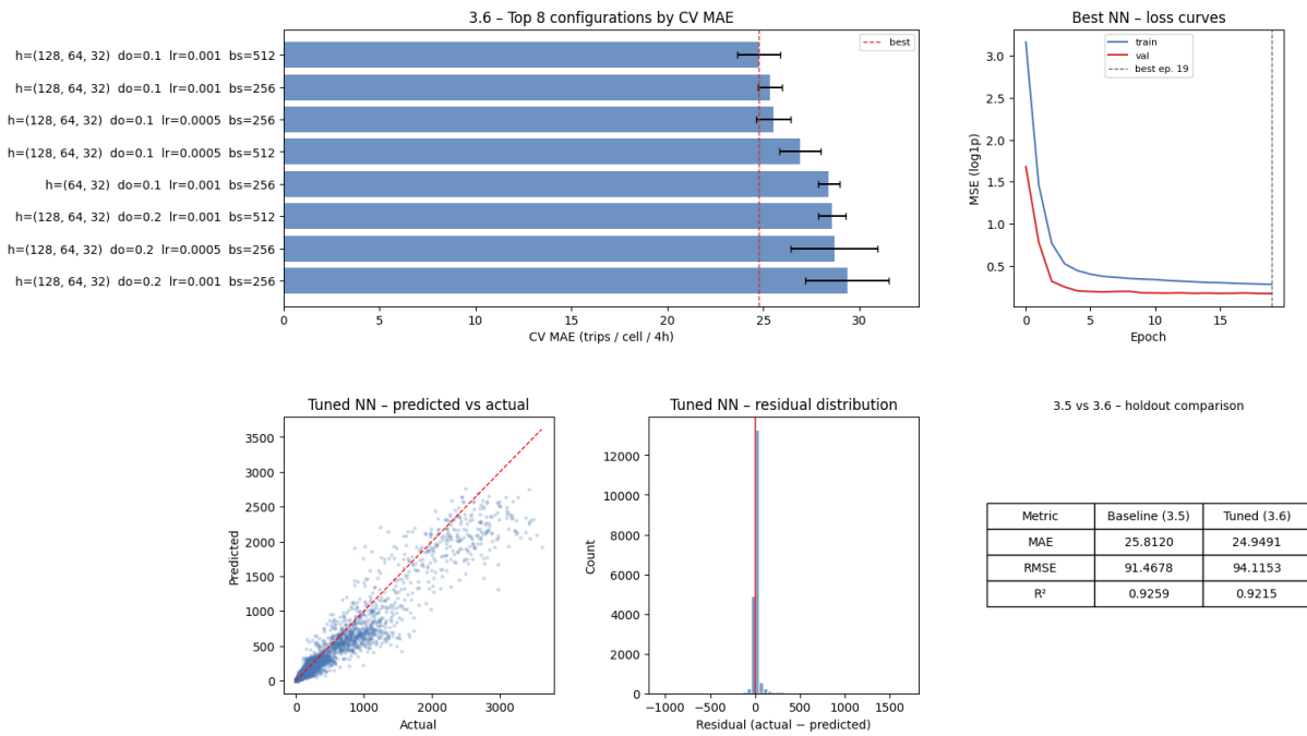
Figure 12: Training result of the tuned neural network, the configuration carried into the holdout comparison.
