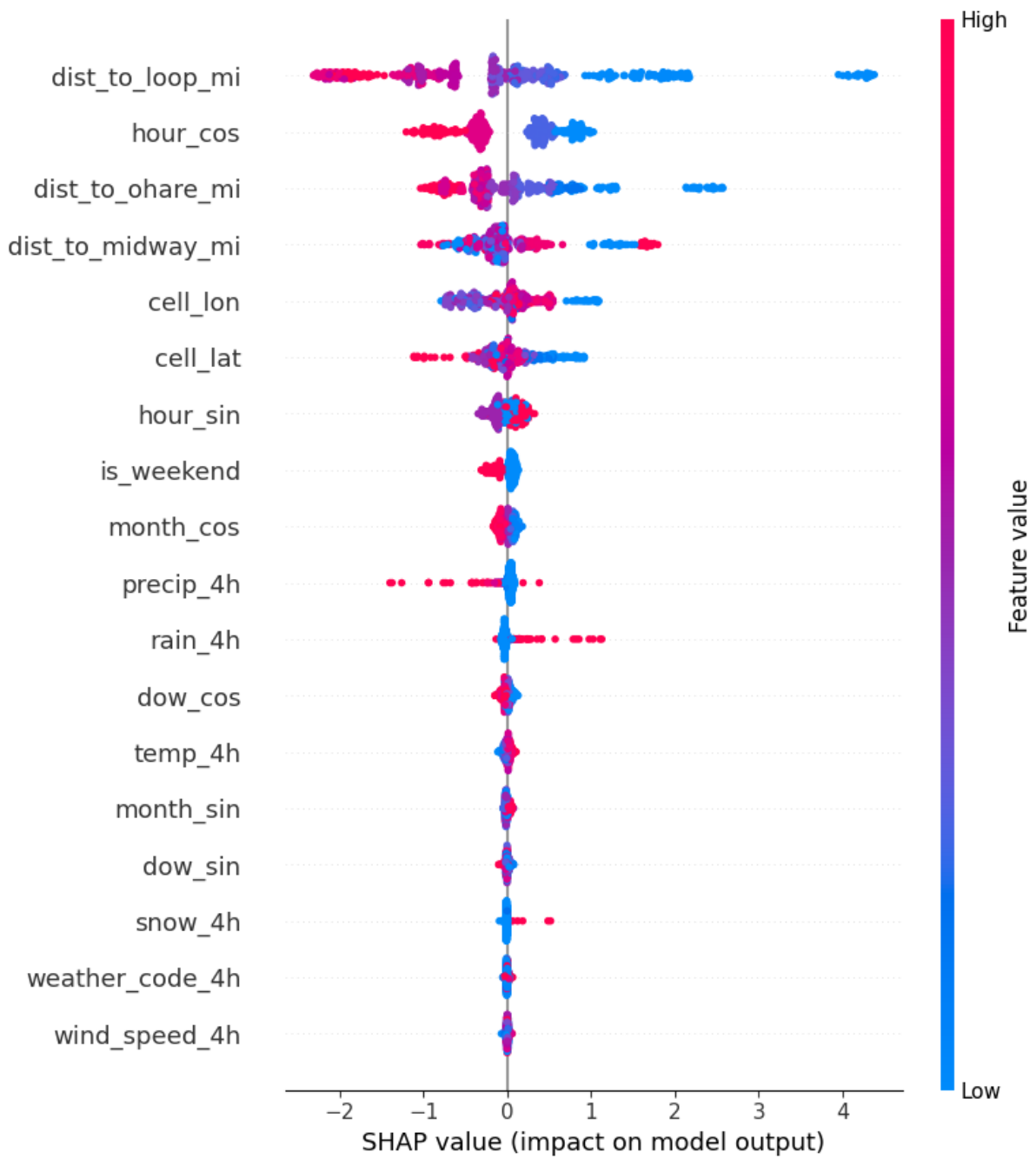
Figure 13: SHAP feature importance for the tuned neural network, showing the distances to the demand centers and the time-of-day terms dominating the prediction.
