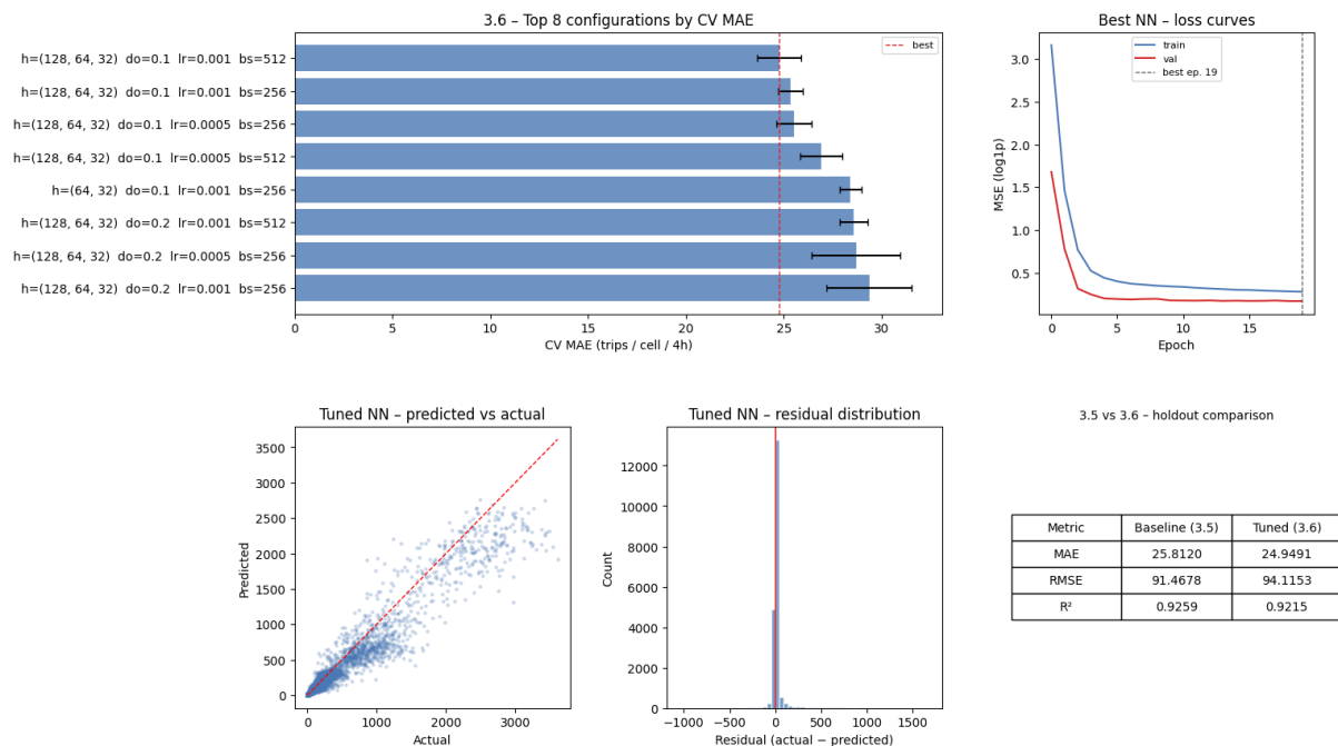
Figure 3: Model result - Neural network tuning model
