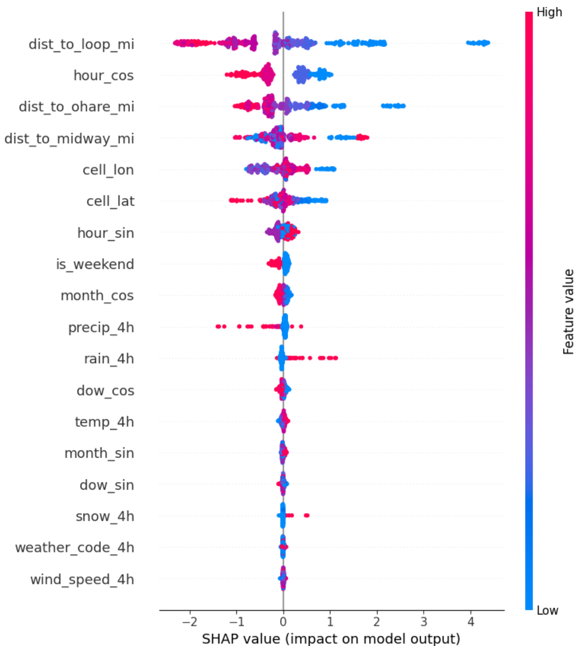
Figure 5: SHAP feature importance
