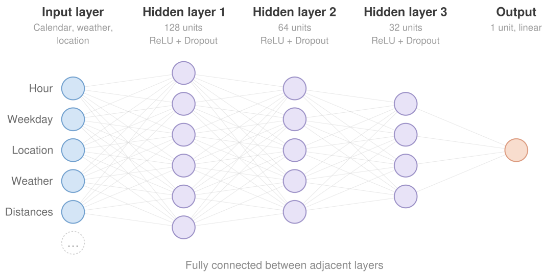
Figure 11: Architecture of the feedforward neural network in its baseline (one hidden layer of 64 units) and tuned (128-64-32) configurations.
