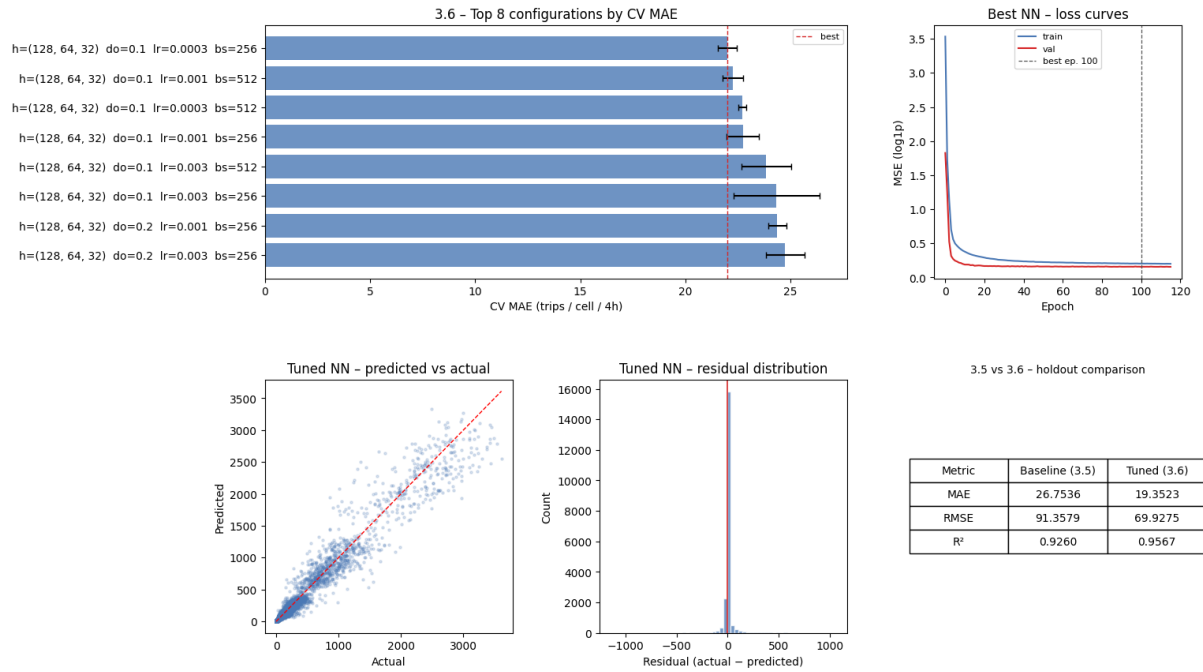
Figure 13: Training result of the tuned neural network.
