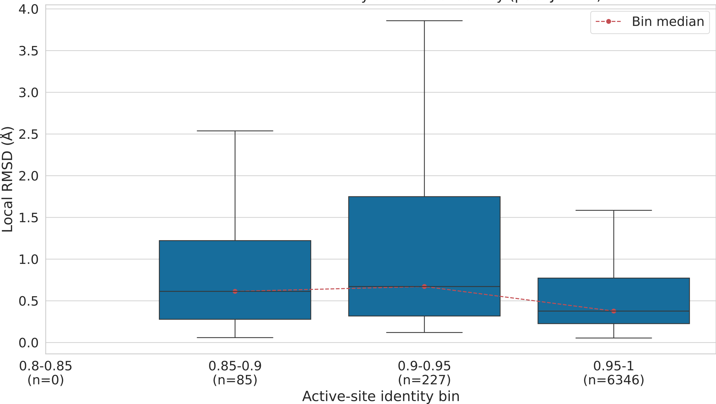
Distribution of Local RMSD by active-site identity (post-JAMDA)
