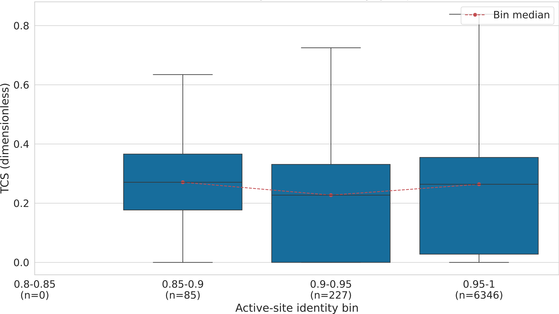
Distribution of TCS by active-site identity (post-JAMDA)
