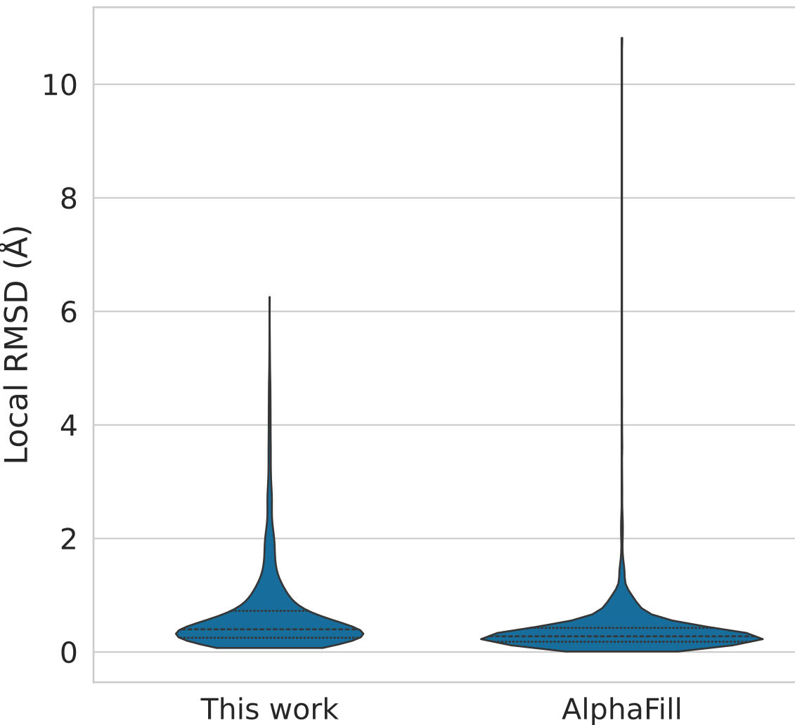
Local RMSD distribution
