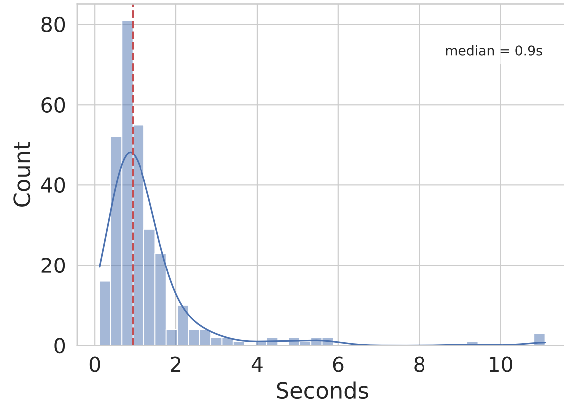
JAMDA runtime (s) (n=265)
