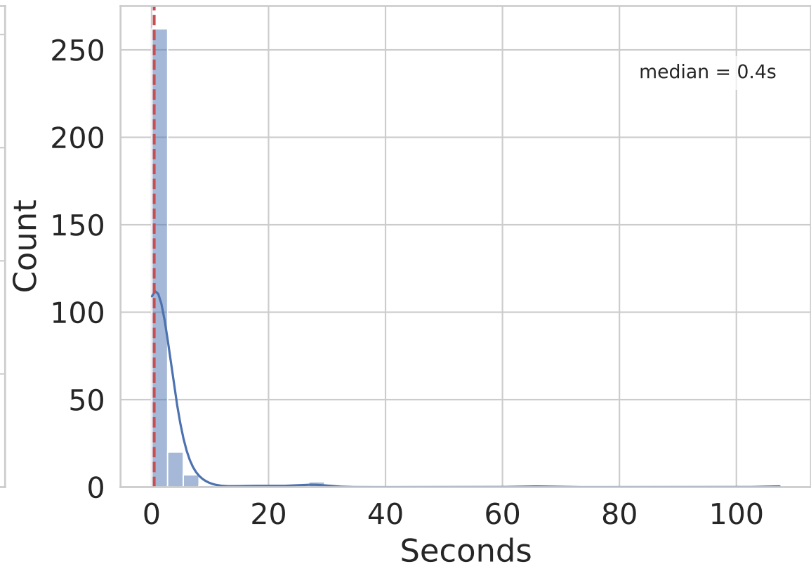
Total pipeline runtime (s) (n=297)
