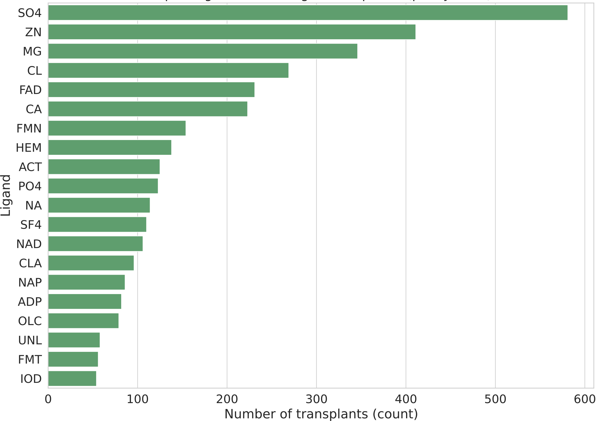
Top 20 ligands excluding buffer species (post-JAMDA)
