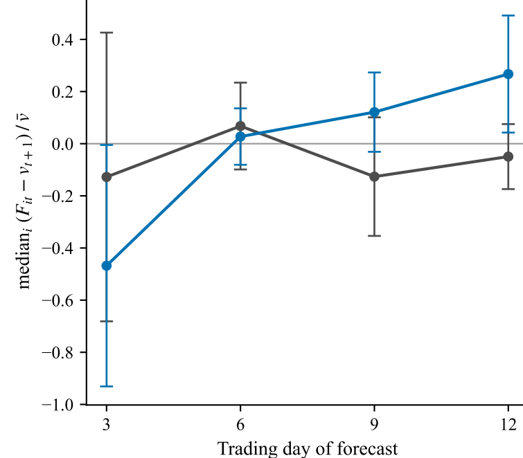
C. Forecast bias vs fundamental
