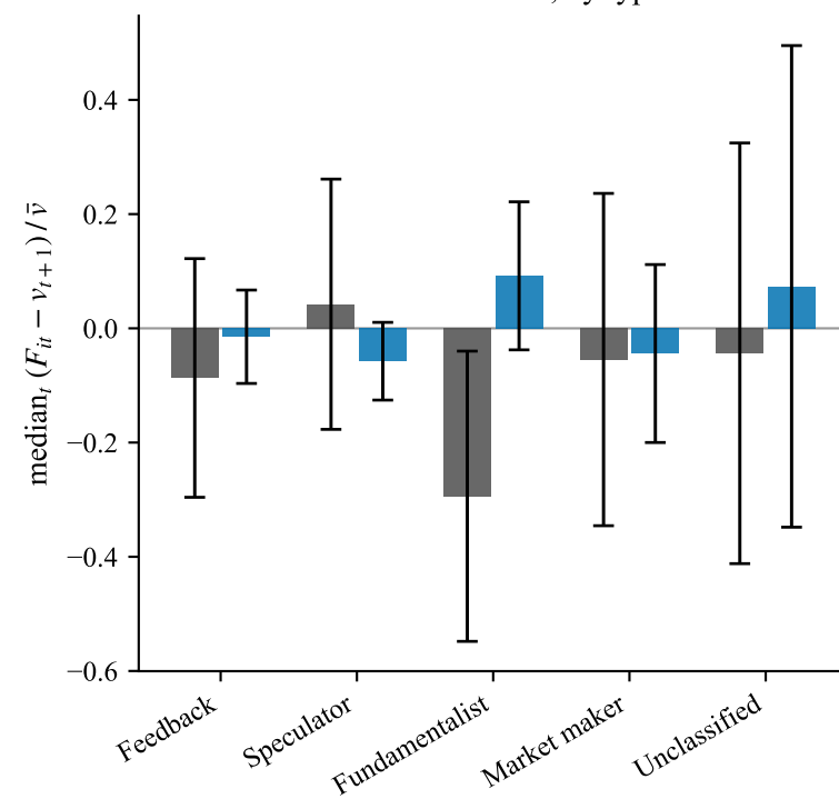
F. Forecast bias vs fundamental, by type
