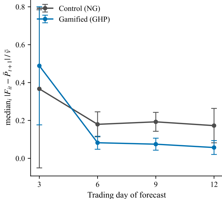
A. Forecast error vs next-day price
