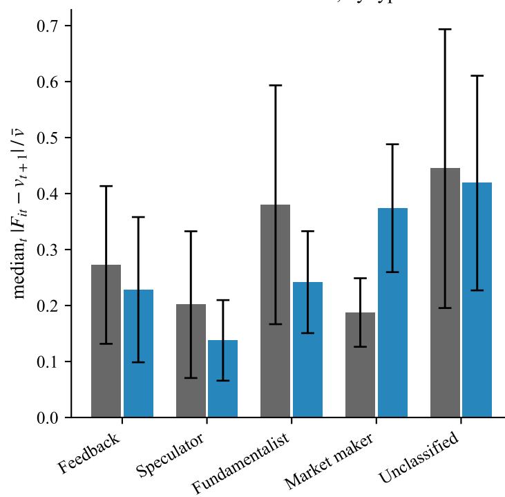
E. Forecast error vs fundamental, by type
