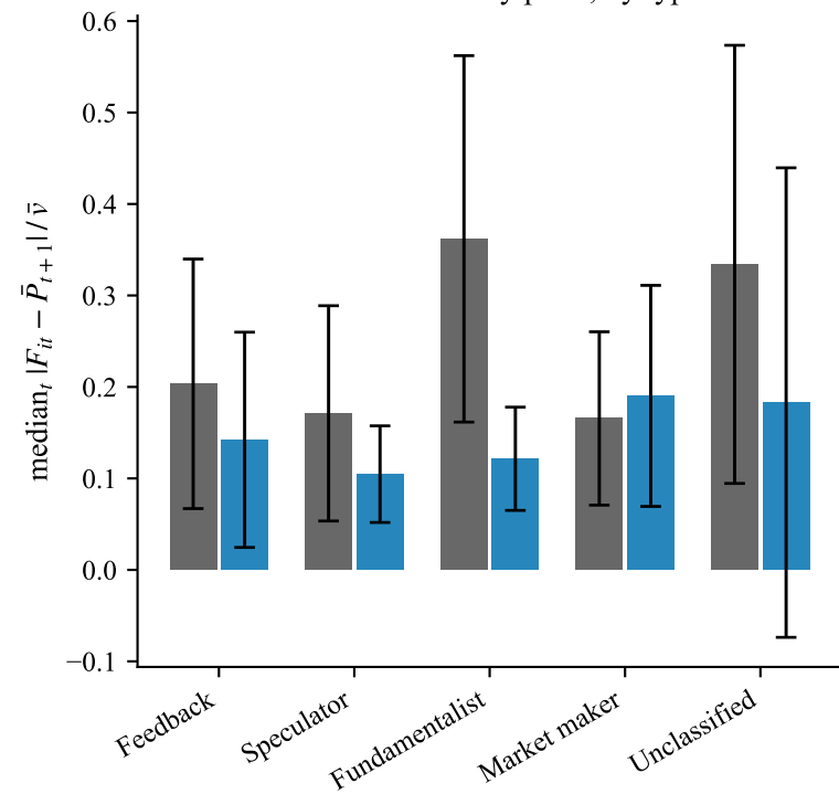
D. Forecast error vs next-day price, by type
