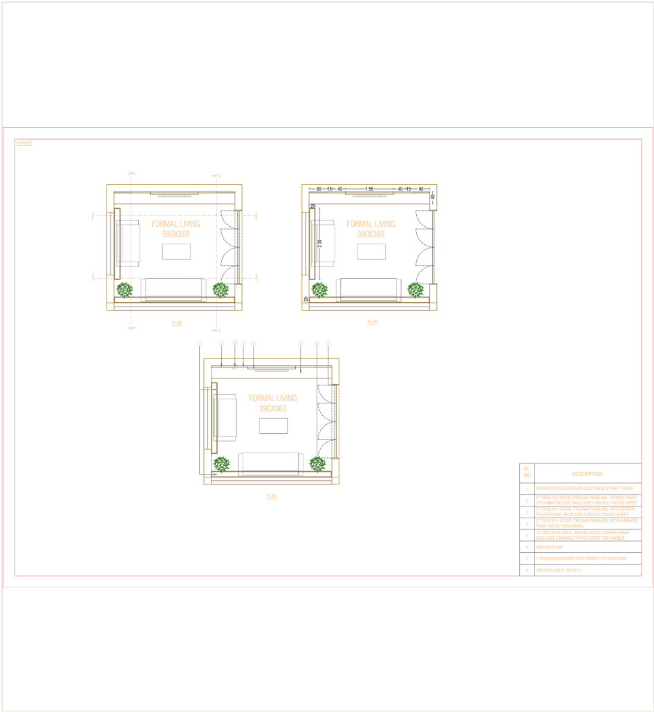
Dimensioned layout detailing circulation corridors, seating positions, masonry envelope, and fenestration openings.
