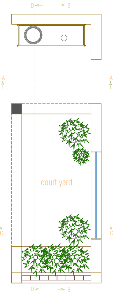
PLAN
