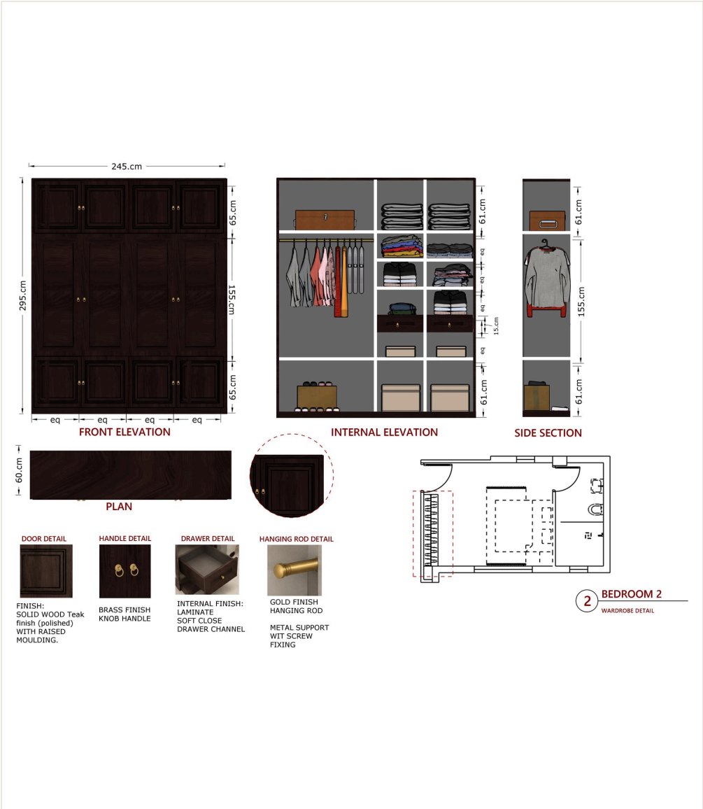
Detailed section through wardrobe units illustrating 18mm marine ply carcass, shelf spacing, and drawer slide positions.
