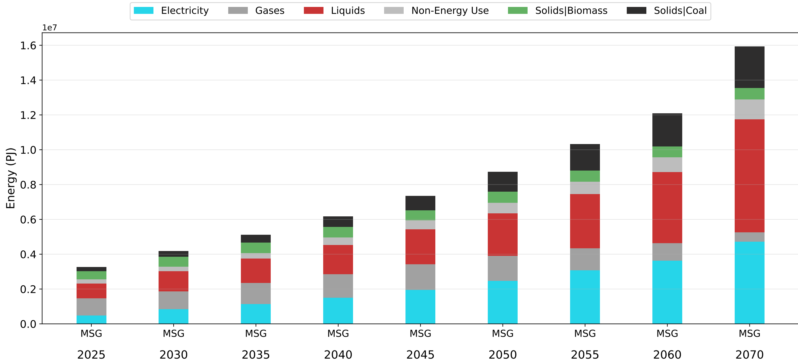
Total Final Energy by Fuel
