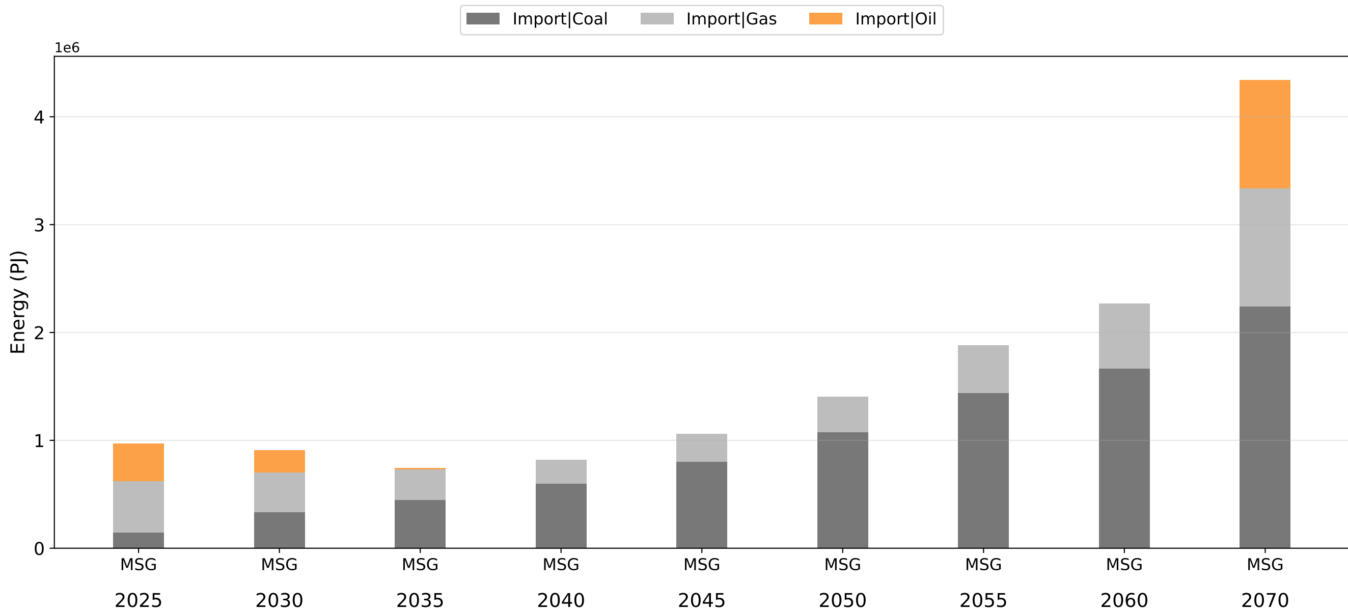
Trade - Primary Energy Volumes
