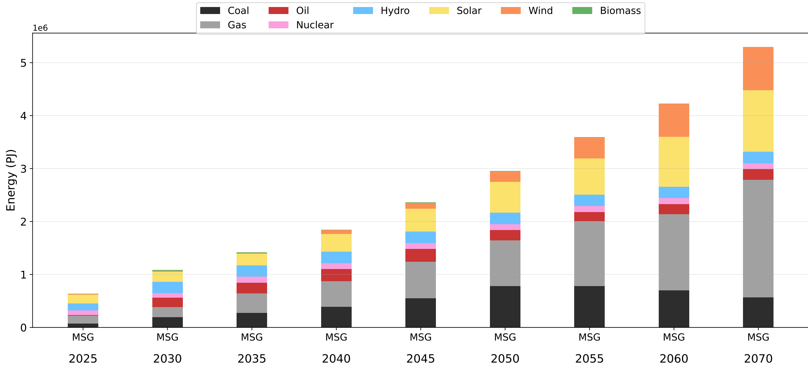
Electricity Generation Mix
