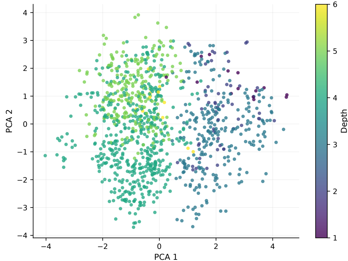
Bilingual structure latent PCA by depth (align 0.10) - seed 0
