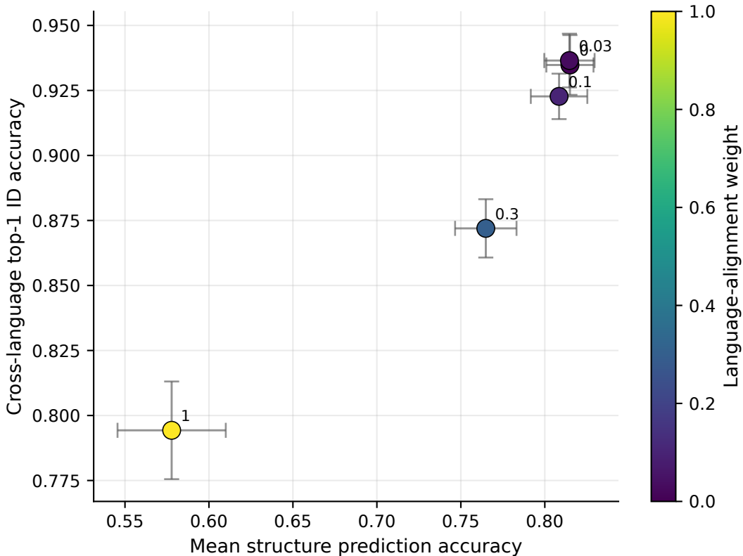
Retrieval-structure tradeoff (seeds 0-9)
