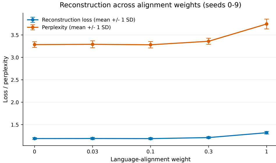
Figure 5. Reconstruction diagnostics across language-alignment weights. Points show means across seeds 0–9, with error bars indicating \pm 1 SD. Reconstruction remains broadly stable at low alignment, but worsens as \lambda increases, especially at \lambda = 1.00 . Reconstruction is therefore a useful diagnostic but not sufficient for model selection.
