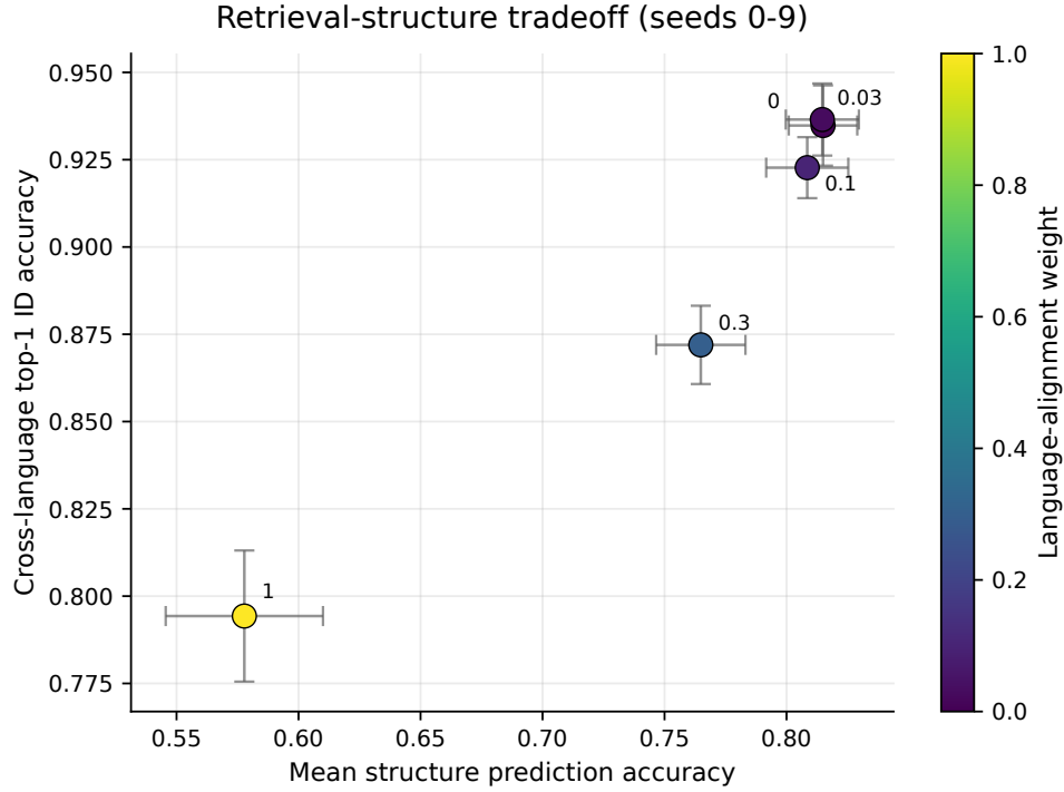
Figure 4. Retrieval-structure trade-off across language-alignment weights. Each point represents the ten-seed mean for a \lambda setting, with error bars showing \pm 1 SD. The x-axis reports mean structure-prediction accuracy from the parent, depth, and next heads; the y-axis reports cross-language Top-1 proposition-ID retrieval. Low alignment occupies the upper-right region, whereas \lambda = 1.00 gives the weakest combined performance.
