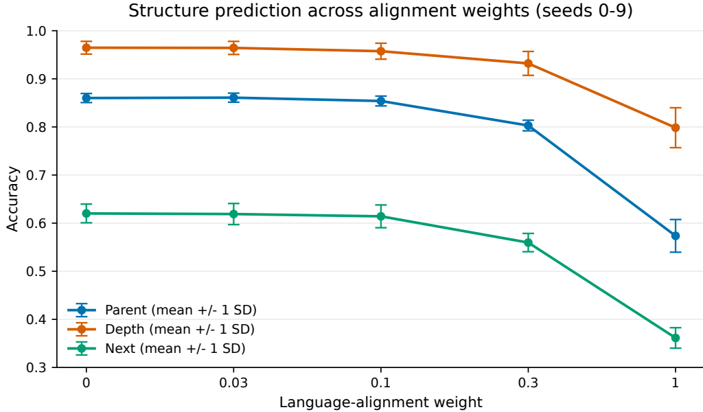
Figure 3. Structure-prediction accuracy across language-alignment weights. Points show means across seeds 0–9, with error bars indicating \pm 1 SD. Depth is recovered most reliably, parent prediction remains strong at low alignment, and next-proposition prediction is the weakest structural task. Stronger alignment steadily degrades all three heads.
