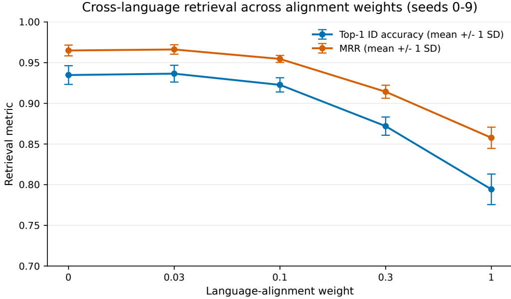
Figure 2. Cross-language proposition retrieval across language-alignment weights. Points show means across seeds 0–9, with error bars indicating \pm 1 SD. Top-1 measures nearest-neighbour same-ID retrieval in the opposite language; MRR measures the rank of the correct match. Retrieval is already strong at \lambda = 0.00 , peaks at \lambda = 0.03 , and declines under stronger alignment.
