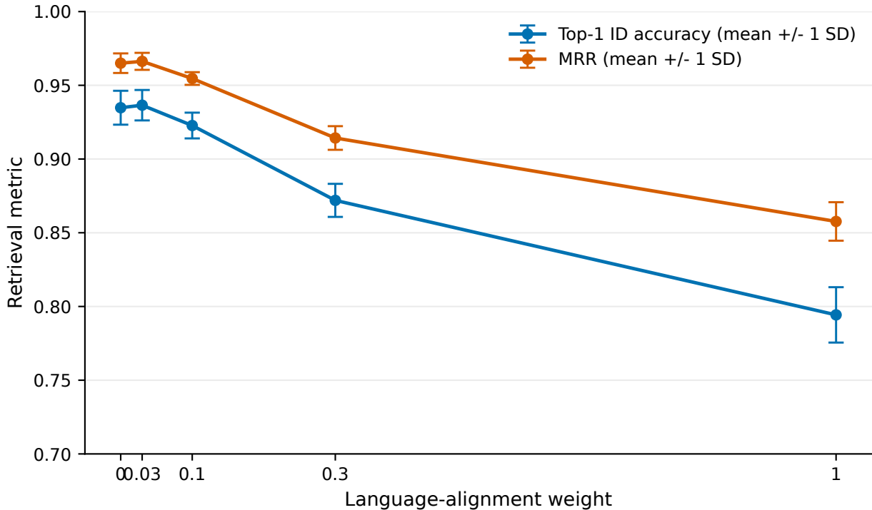
Cross-language retrieval across alignment weights (seeds 0-9)
