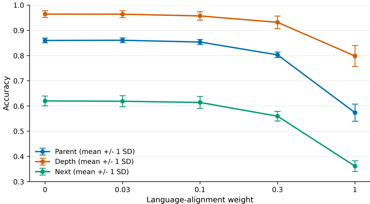
Structure prediction across alignment weights (seeds 0-9)
