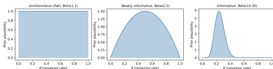
Figure 9.2.: Three types of prior belief about a response rate, from no opinion (flat) to a confident prior expectation (informative).
