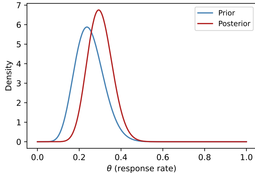
Informative: Beta(10,30)
