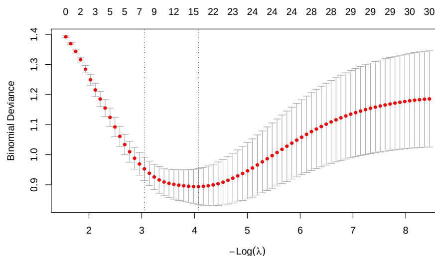
Figure 7.5.: Cross-validation curve for LASSO. The x-axis is -\log(\lambda) (so the penalty decreases left to right), the y-axis is cross-validated deviance. Vertical lines mark \lambda_{1se} (left) and \lambda_{min} (right).
