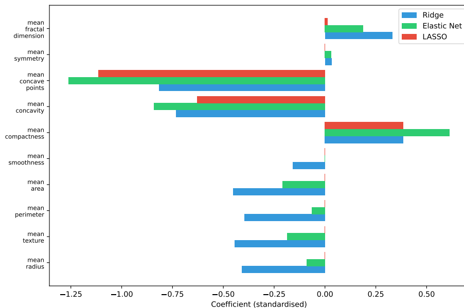
Figure 7.8.: Coefficient estimates from Ridge, Elastic Net, and LASSO for the breast cancer dataset (Python). Ridge retains all predictors; LASSO sets many to zero; Elastic Net is intermediate.
