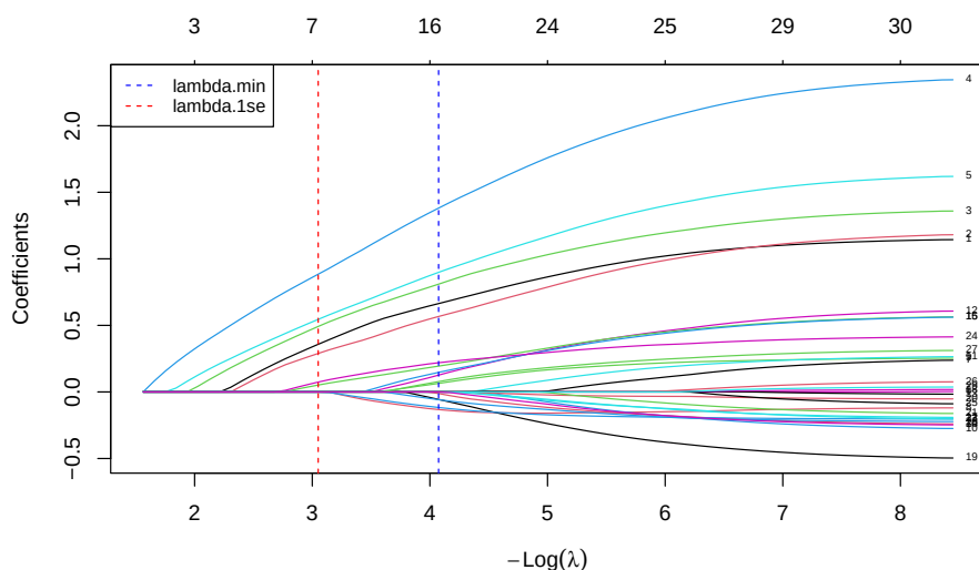
Figure 7.6.: LASSO regularisation path. Each line is one coefficient. As lambda decreases (left to right), more coefficients become non-zero. The five truly non-zero coefficients (shown as they enter the model) are recovered first.
