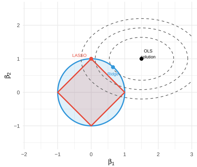
Figure 7.4.: Geometric comparison of L1 (LASSO, diamond) and L2 (Ridge, circle) constraints. The ellipses are contours of the loss function. The LASSO solution hits the corner of the diamond, setting one coefficient to zero.
