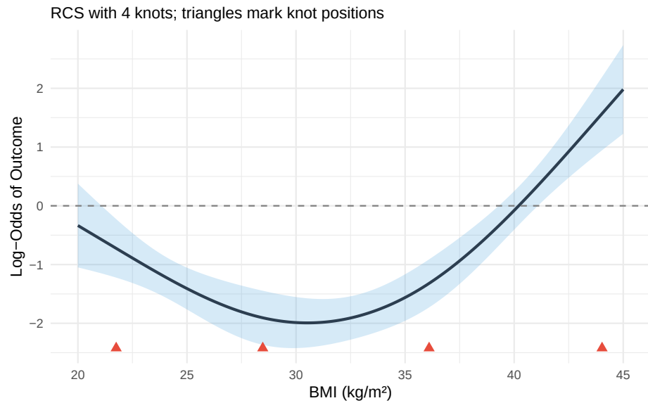
Figure 6.2.: Illustration of an RCS(4) fit. Knot locations are marked with triangles. The relationship is linear beyond the outer knots and flexibly curved between them.
