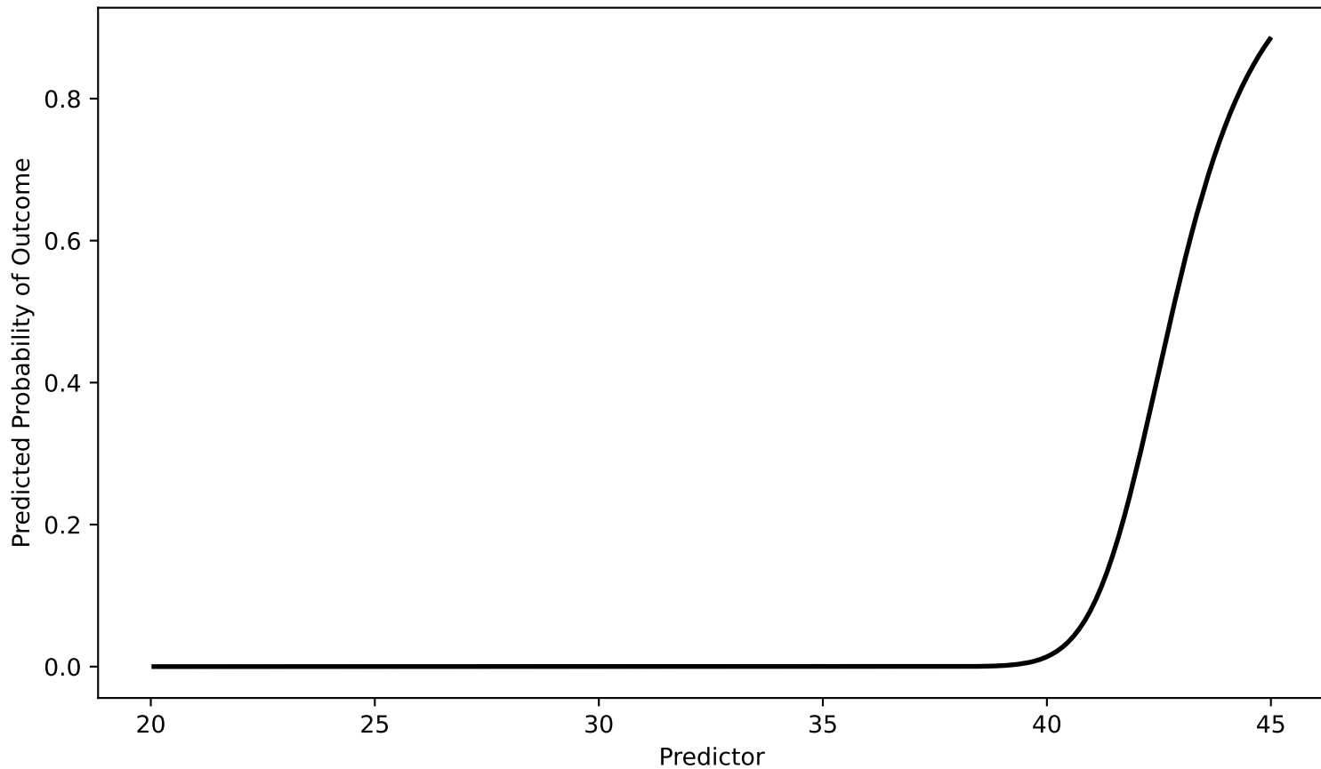
Non-linear relationship modelled with a restricted cubic spline
