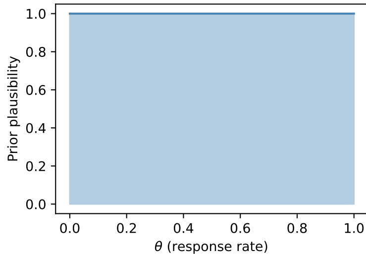
Uninformative (flat): Beta(1,1)
