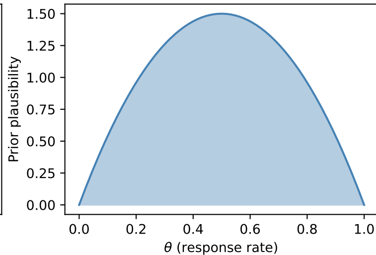
Weakly informative: Beta(2,2)
