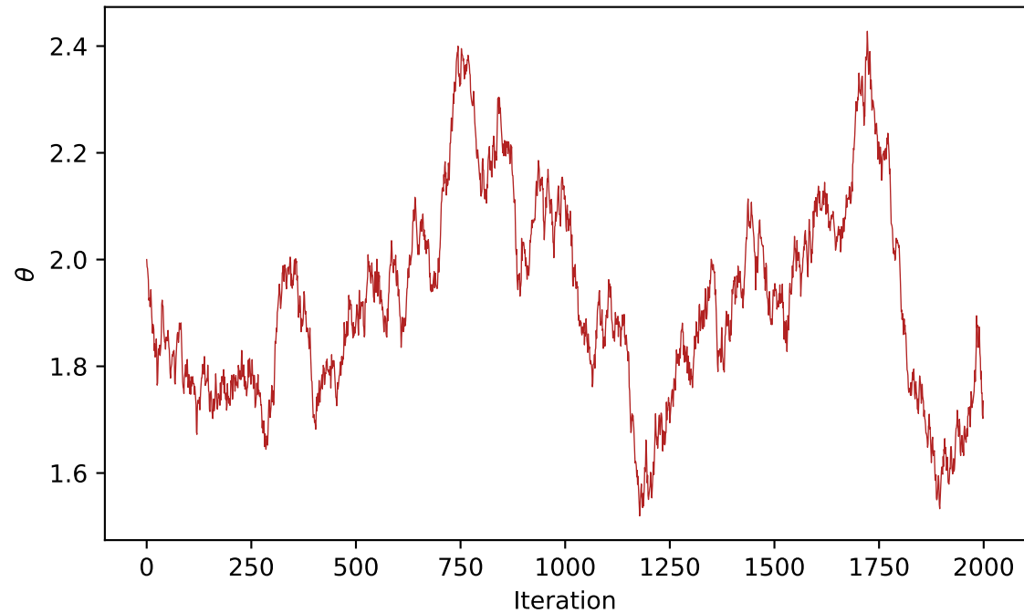
Poor mixing
