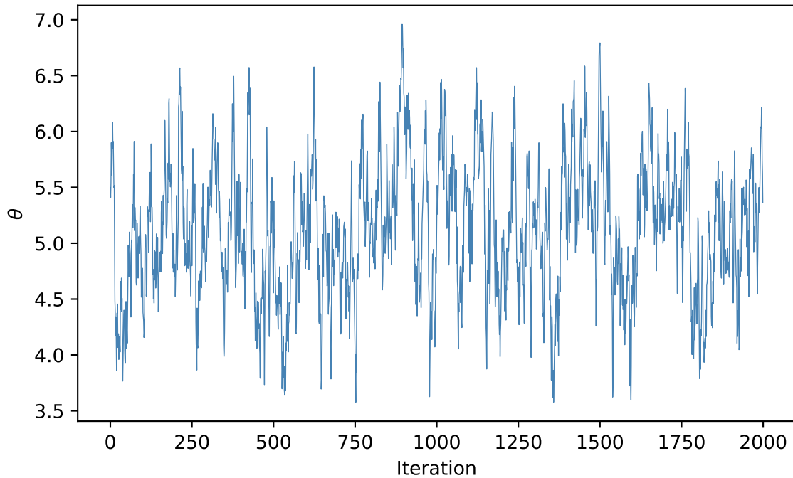
Good mixing
