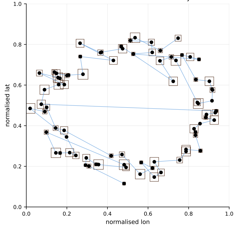
BR-LZ data structure: 80 OSM MBRs sorted by Z-order
